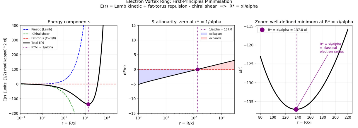
Figure 1: Electron vortex ring energy landscape. Left: The three contributions to \mathcal{E}(r) (16) in units of \frac{1}{2}\rho_0\kappa_0^2\xi : kinetic/Lamb (blue dashed), chiral-shear resistance (green dashed, negated), and fat-torus repulsion 2C/r (red dashed), with total \mathcal{E} (black). Centre: The stationarity condition d\mathcal{E}/dr changes sign exactly at r^* = 1/\alpha = 137 . Right: Zoom near the minimum confirming a well-defined bound state at R_e^* = \xi/\alpha (the classical electron radius). Computed with \alpha = 1/137.036 .
